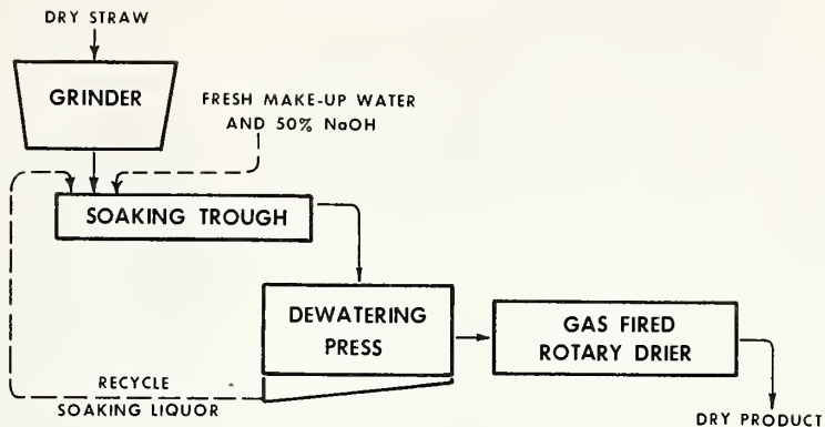
Fig. 4. Alkali soaking.
